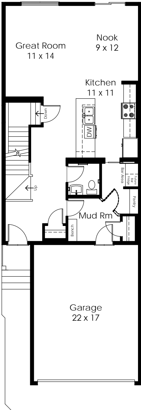
Main Floor 836 sqft Option B - Bar Area
