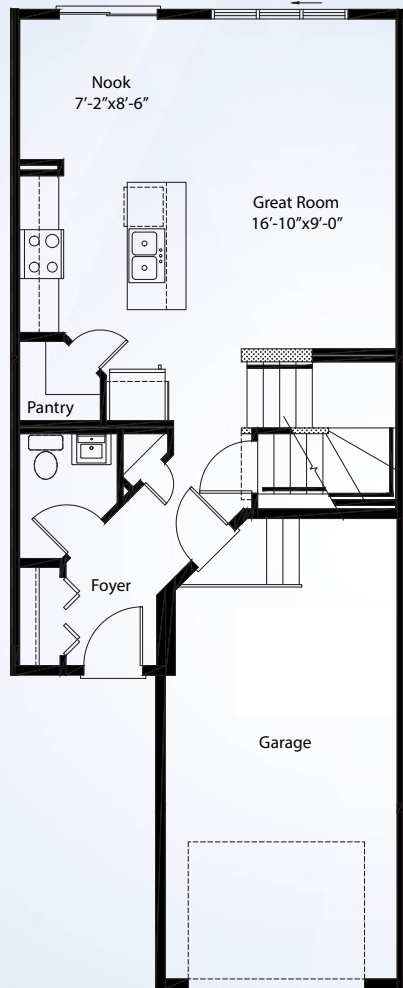
Main Floor | 593 Sq. Ft.
